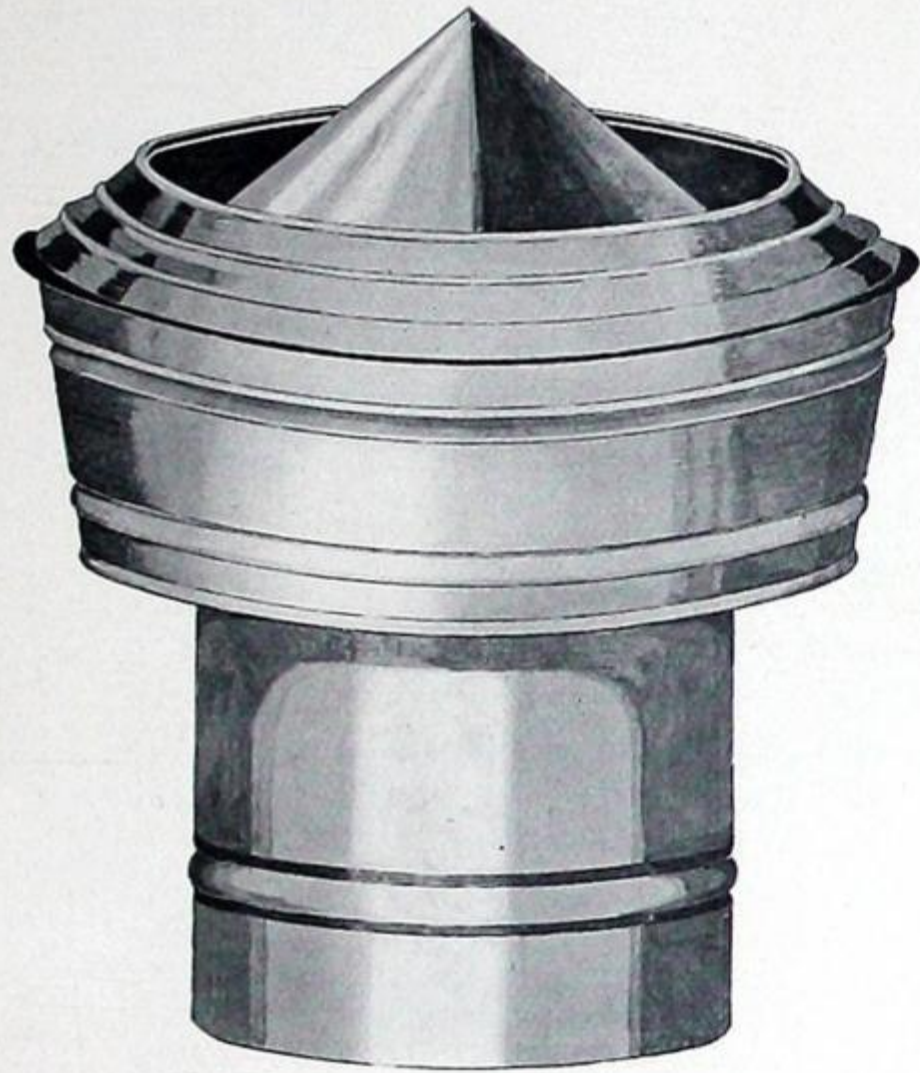
Fig. 227.—Complete View of Ventilator.
